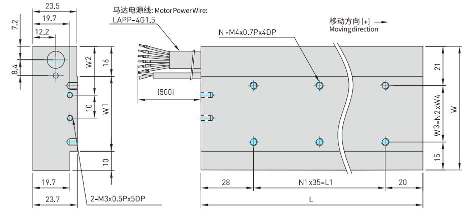
TPA-P 动子尺寸图 TPA-P moving size diagram
