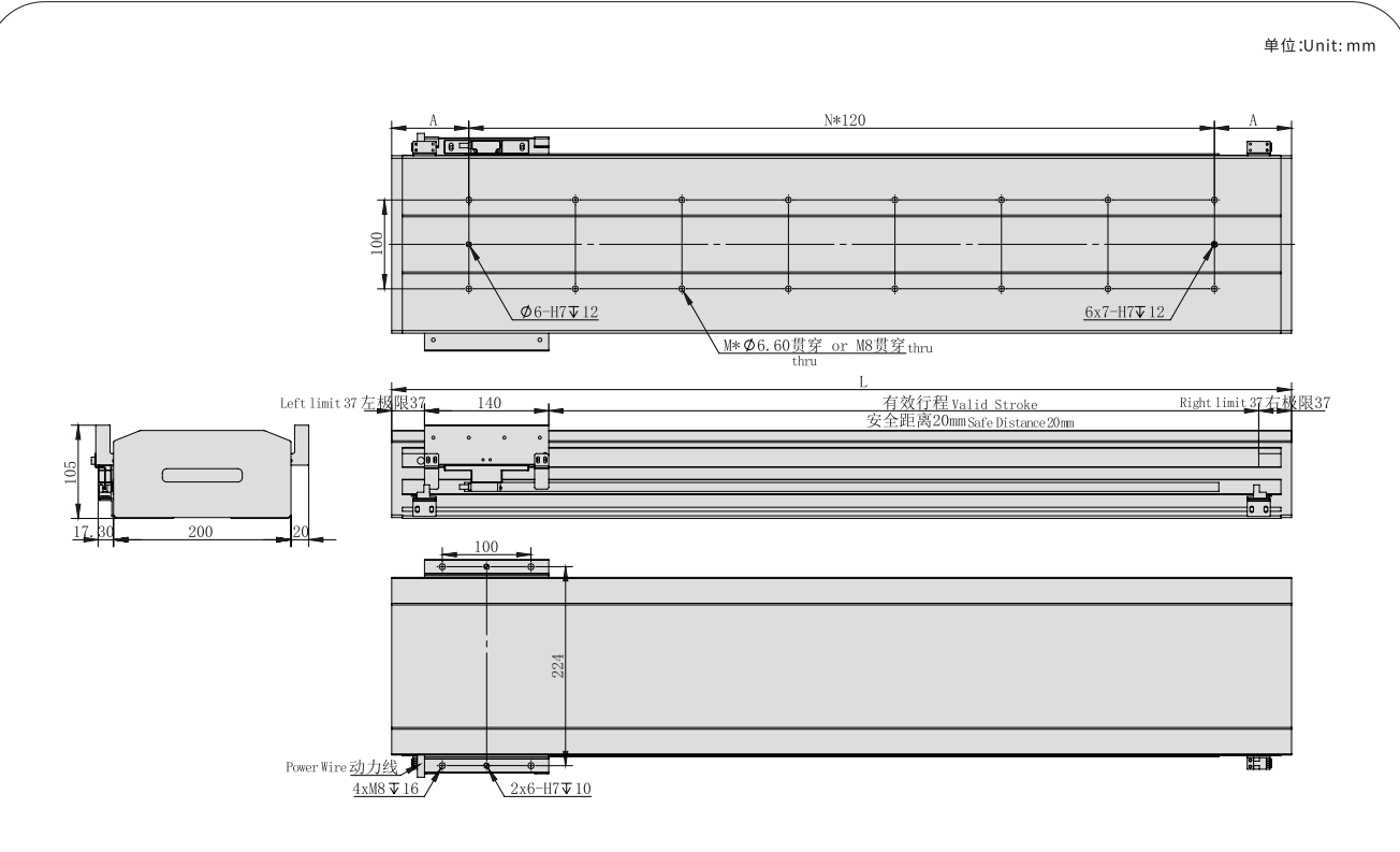
TPA-LNP-200-P21--512N直线电机 TPA-LNP-200-P21--512N Linear motor
