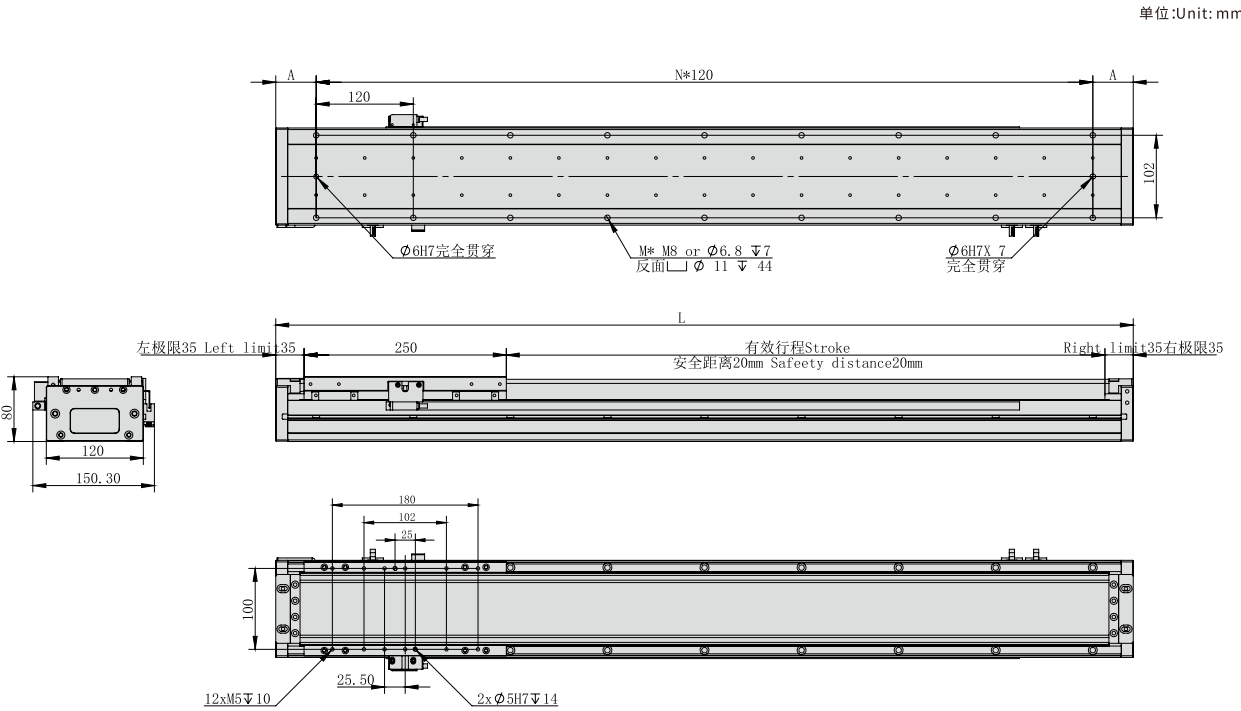
TPA-LNP3-120-35C4--532N直线电机 TPA-LNP3-120-35C4--532N Linear motor
