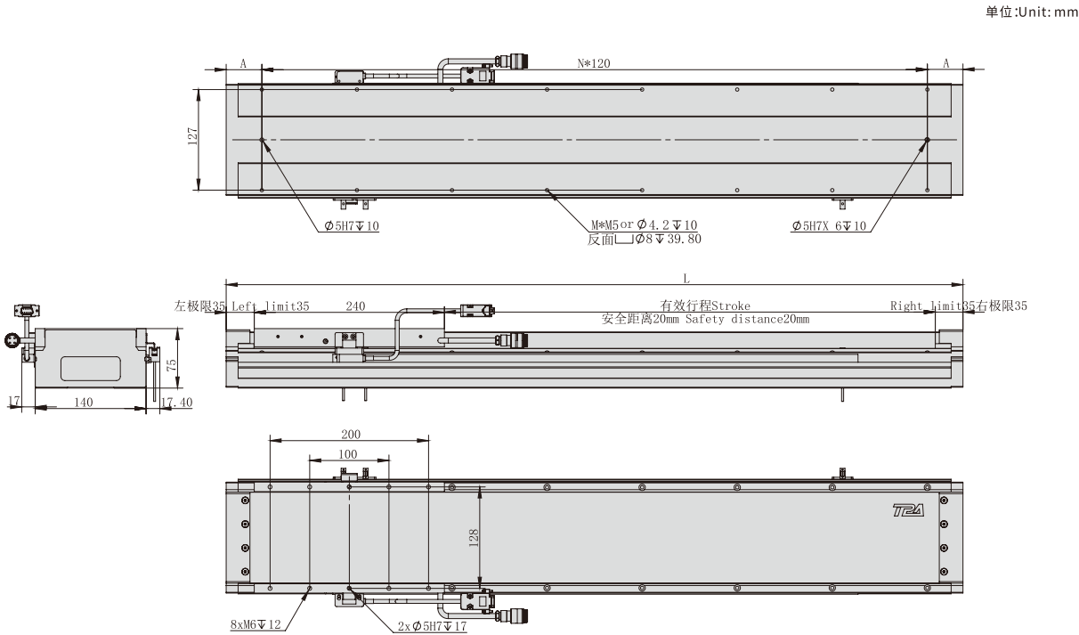
TPA-LNP2-140-20C4--301N直线电机 TPA-LNP2-140-20C4--301N Linear motor
